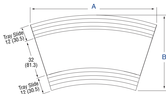
Top View – Base Plus Two Tray Slides
