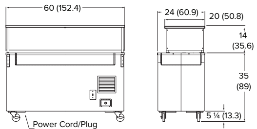
4-Pan Refrigerated Cold Station with NSF2 Buffet Breath Guard
