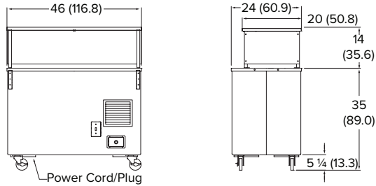
3-Pan Refrigerated Cold Station with NSF2 Buffet Breath Guard
